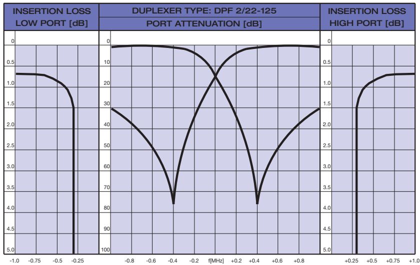
TYPICAL RESPONSE CURVES @ 0.8 MHz DUPLEX SPACING:
