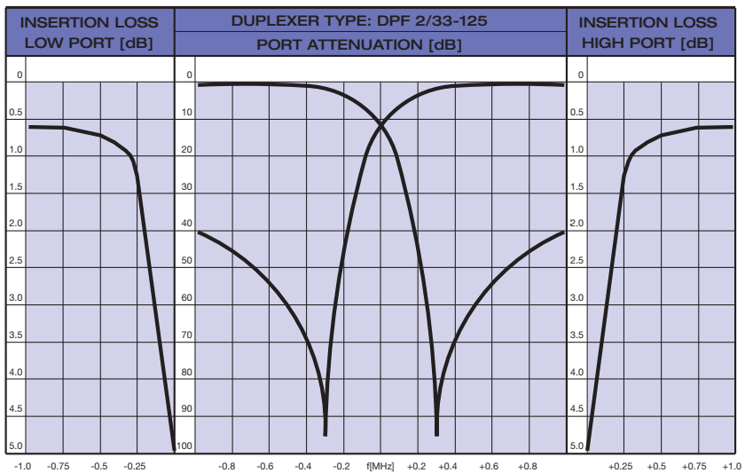
TYPICAL RESPONSE CURVES @ 0.6 MHz DUPLEX SPACING:
