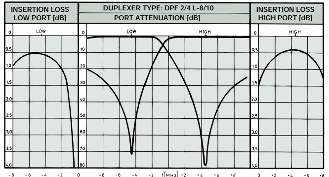
TYPICAL RESPONSE CURVES @ 9 MHz DUPLEX SPACING:
