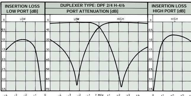
TYPICAL RESPONSE CURVES @ 4.5 MHz DUPLEX SPACING:
