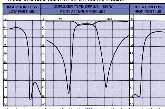
TYPICAL RESPONSE CURVES @ 4.5 MHz DUPLEX SPACING:
