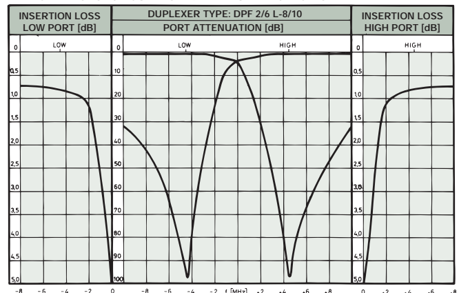
TYPICAL RESPONSE CURVES @ 9 MHz DUPLEX SPACING:
