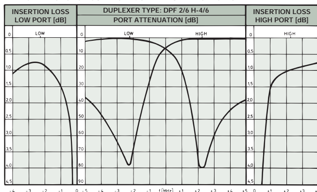
TYPICAL RESPONSE CURVES @ 4.5 MHz DUPLEX SPACING:
