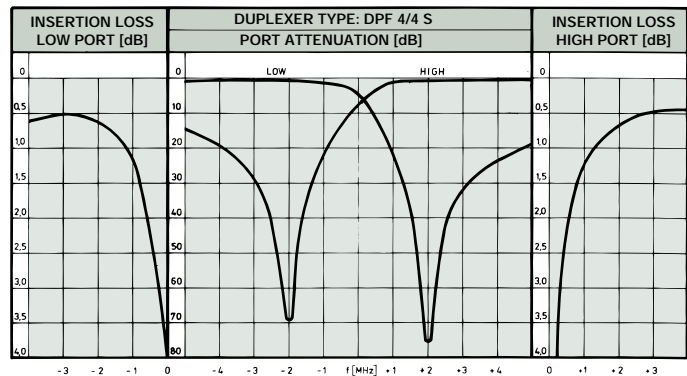
TYPICAL RESPONSE CURVES @ 4 MHz DUPLEX SPACING:
