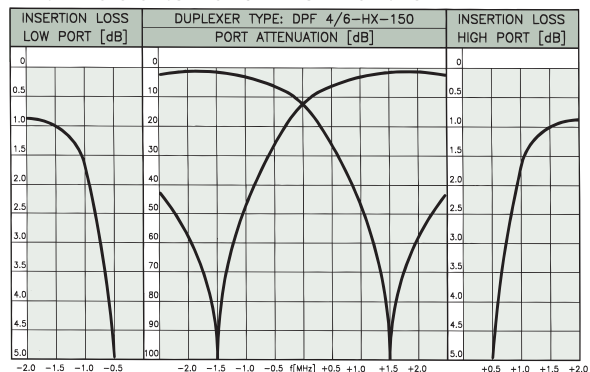
TYPICAL RESPONSE CURVES @ 3 MHz DUPLEX SPACING:
