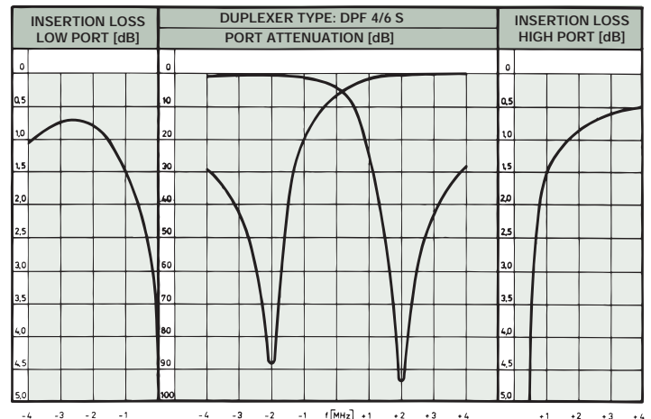
TYPICAL RESPONSE CURVES @ 4 MHz DUPLEX SPACING:
