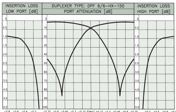
TYPICAL RESPONSE CURVES @ 1 MHz DUPLEX SPACING:
