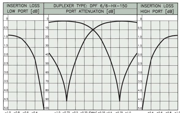
TYPICAL RESPONSE CURVES @ 1.5 MHz DUPLEX SPACING:
