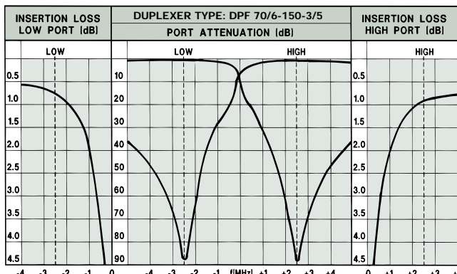
TYPICAL RESPONSE CURVES SPACING = 5 MHz
