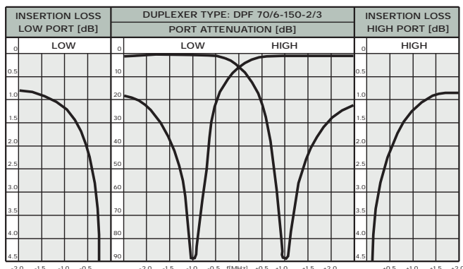
TYPICAL RESPONSE CURVES SPACING = 2 MHz
